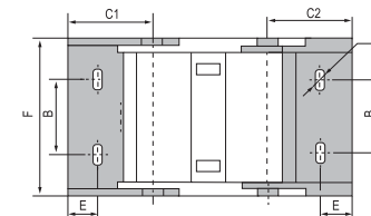
X 2 型接头 X 2 type bracket
